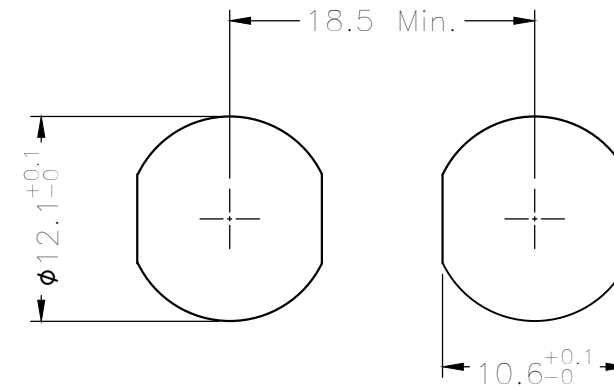
PANEL CUT-OUT
