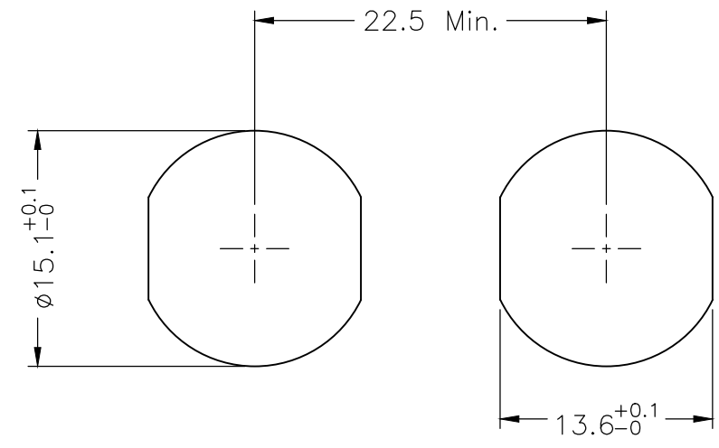
PANEL CUT-OUT
